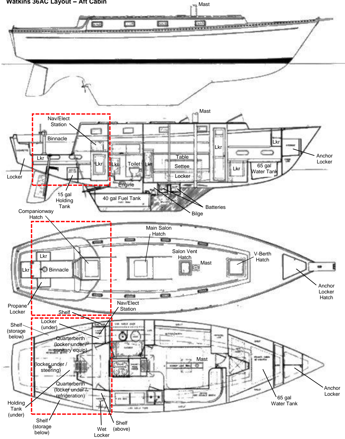
Aft Cabin
